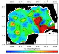
Real-Time Mesoscale Altimetry - May 18, 2010
