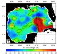
Real-Time Mesoscale Altimetry - Apr 22, 2010
