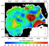
Real-Time Mesoscale Altimetry - Jun 12, 2010
