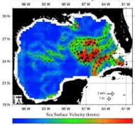
Real-Time Mesoscale Altimetry - Jun 12, 2010
